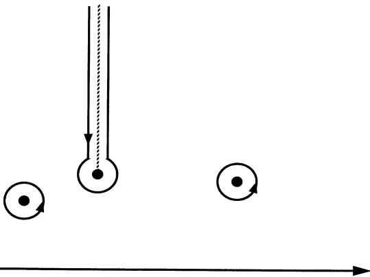
FIG. 1. Moving the contour to surround singularities in the upper half-plane.
