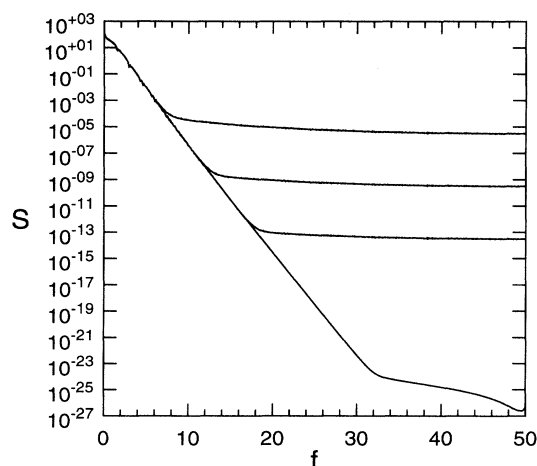
FIG. 2. Power spectra, S , versus frequency, f , from the time series of the variable x from the Lorenz model for four noise values ( \mu = 0, 2.5 \times 10^{-1}, 2.5 \times 10^{-3}, and 2.5 \times 10^{-5} ). See Sec. VIB for details of the model and computations.
