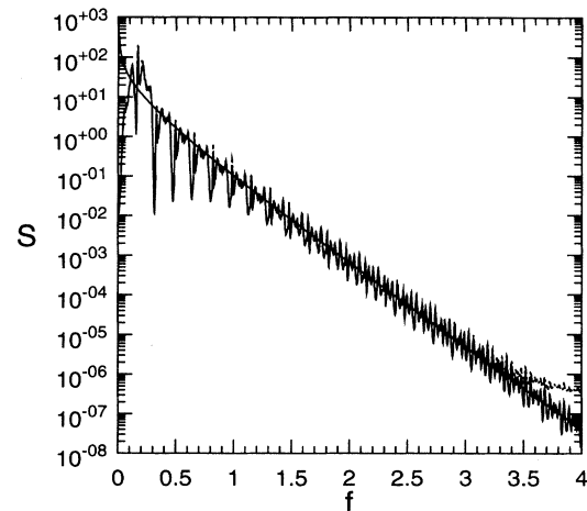
FIG. 9. Low-noise, zero-noise, and asymptotic spectra, S , versus frequency, f , from time series of the variable x from the Rossler model. The rough, solid curve is the zero-noise spectrum. The dashed curve—which is distinguishable from the rough, solid curve only in the lower right corner of the figure—is the low-noise spectrum. The smooth solid curve is a function of the form Cf^n e^{-kf} where the parameters C , n , and k have been fit to the zero-noise spectrum in the region where the spectrum has clearly become asymptotic. The frequency is in inverse model time units. See Sec. VIC 2 for details of the computation of the spectra including details of the normalization.
